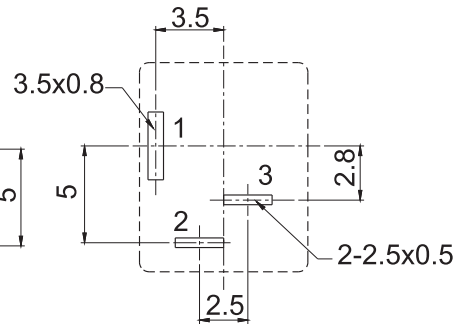
P.C.B Layout(Copper-side view)
