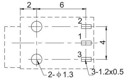
P.C.B Layout(copper-sided view)
