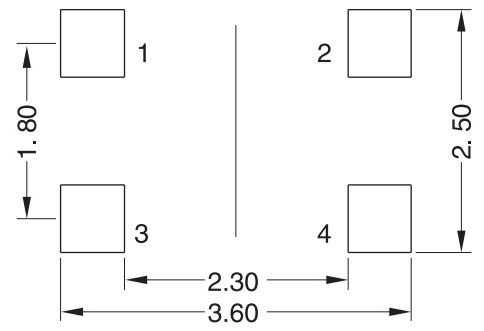
Recommended PAD Layout \phi+0.05 TOP VIEW
