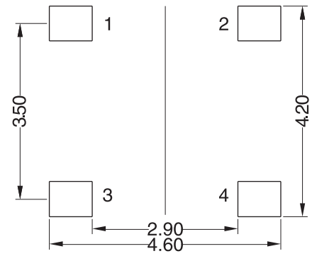
Recommended PAD Layout \oplus 0.05 TOP VIEW
