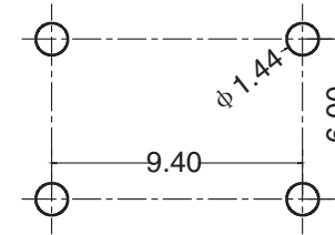
PCB Layout Recommended
